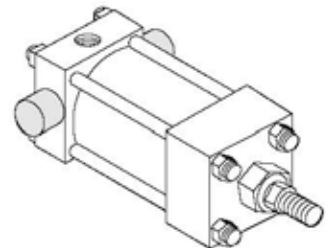
Code WS (MT2) Cap Trunnion
