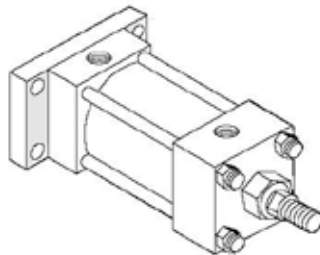
Code RS (MF2) Cap Rectangular Flange
