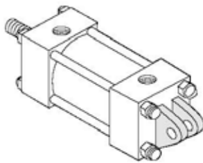
Code CF (MP1) Cap Fixed Clevis
