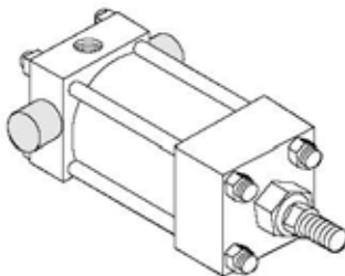
Code WS (MT2) Cap Trunnion
