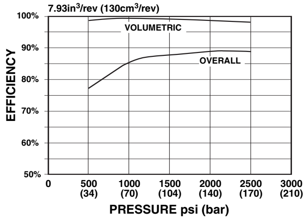
EFFICIENCY @ 1800 rpm
