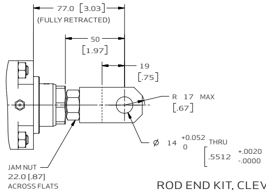
ROD END KIT, CLEVIS END OPTION (CODE: 3)
